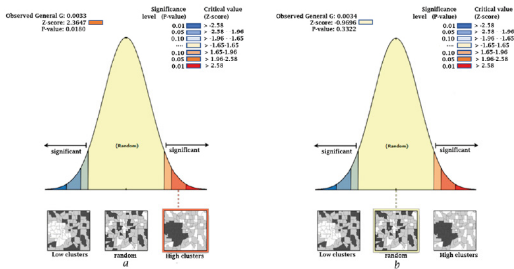
Figure 7. Getis-Ord index for pH and TSS variables. Figure 7.a Getis-Ord index for pH week 5. Figure 7.b Getis-Ord index for TSS week 4. (own source)
