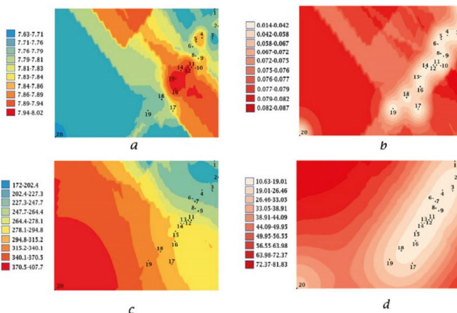
Figure 4. pH and TSS prediction and error surfaces, using Ordinary Kriging. Figures 4.a and 4.b show prediction and error surfaces for pH week 5. Figures 4.c and 4.d show prediction and error surfaces for TSS week 4. (own source)
