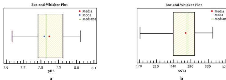
Figure 2. Box and whisker plots. a) Box and whisker plot pH week 5. b) Box and whisker plot TSS variable week 4. (own source)
