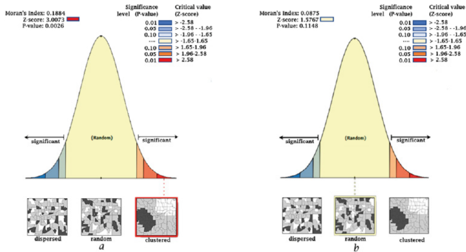
Figure 6. Moran's index source ArcGIS 10.7 for the pH and TSS variables. Figure 6.a Moran's index for pH week 5. Figure 6.b Moran's index for TSS week 4. (own source)
