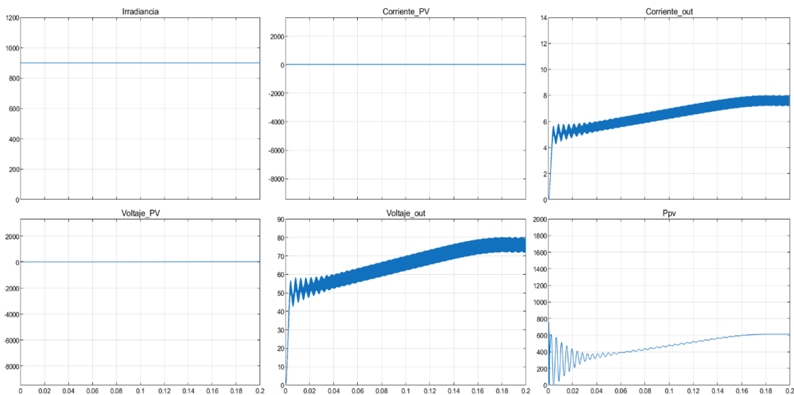
Figura 17: Salida P&O paso variable.
